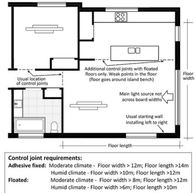
Figure 2 – Installation
