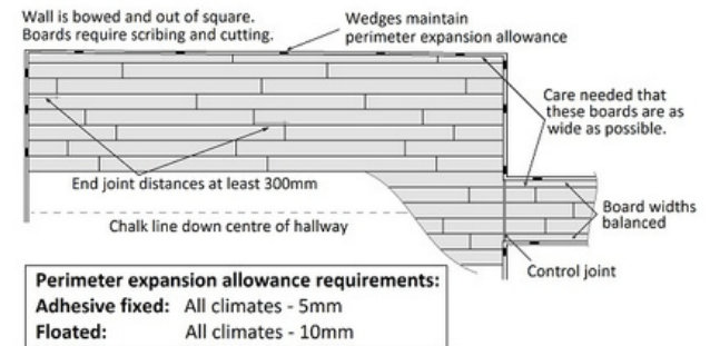
Figure 3 – Scribing
